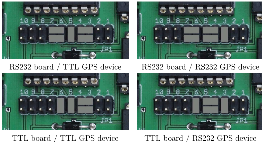
Figure 20: Jumper JP1.
