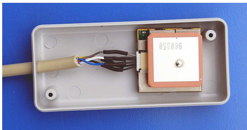
Figure 37: An EM-406A module embeddet into a plastic housing.
