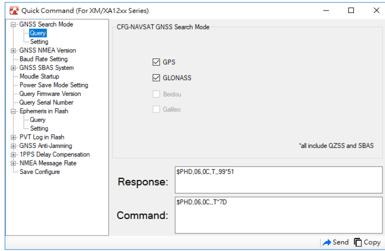
Figure 2-52: Quick Command Window for XA12xx and XM12xx
