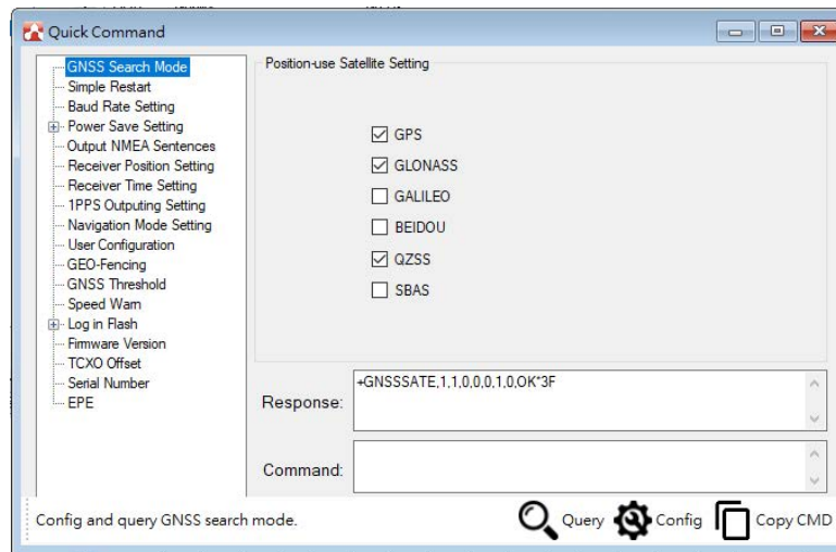
Figure 2-53: Quick Command Window for XP2210 and XS1110
