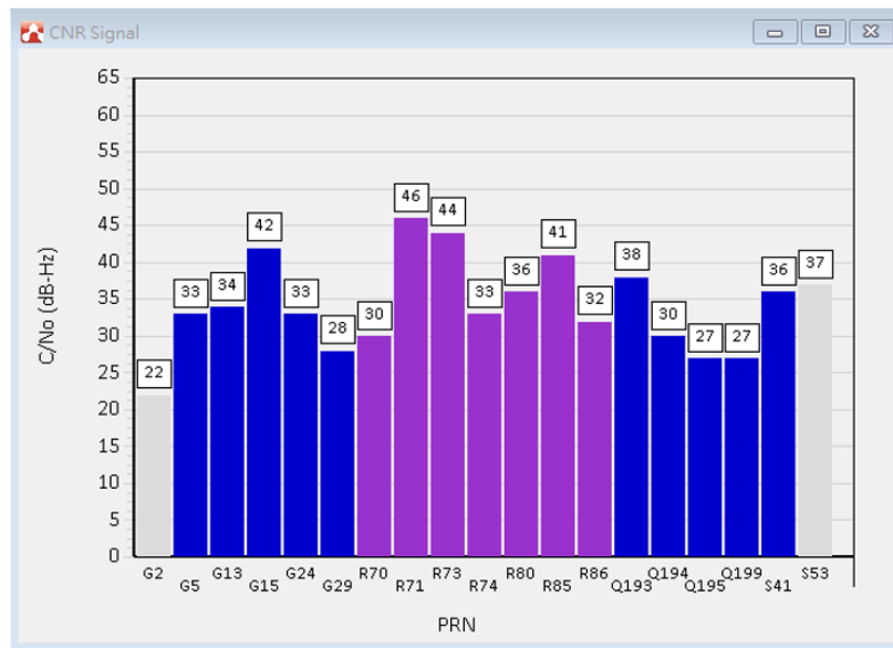
Figure 2-33: CNR Signal Window (GPS+GLONASS)
