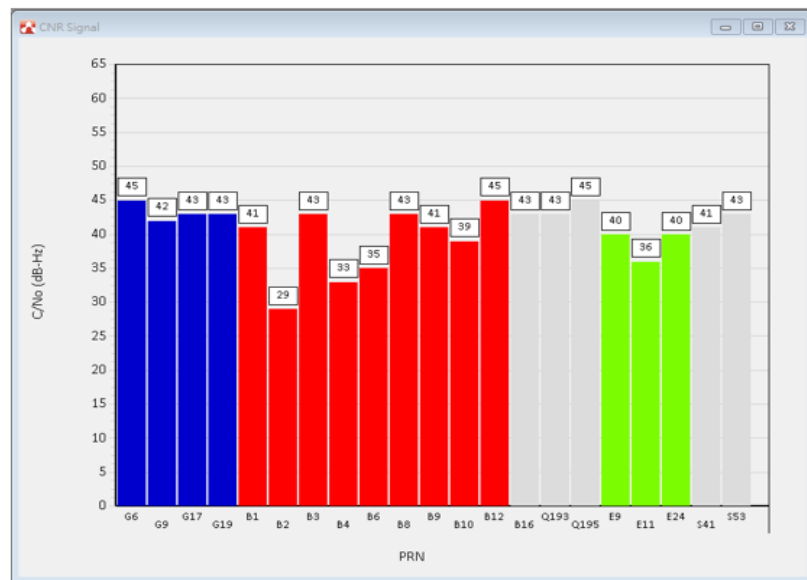
Figure 2-34: CNR Signal Window (GPS+Beidou+Galileo)
