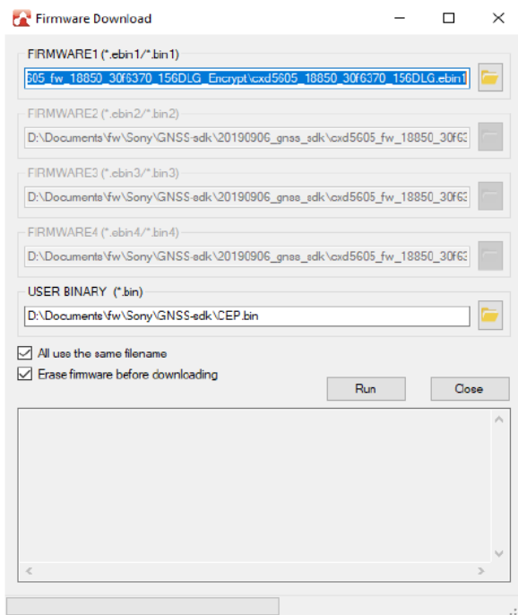
Figure 2-14: Download ROM Dialog (For XP2210 and XS1110)
