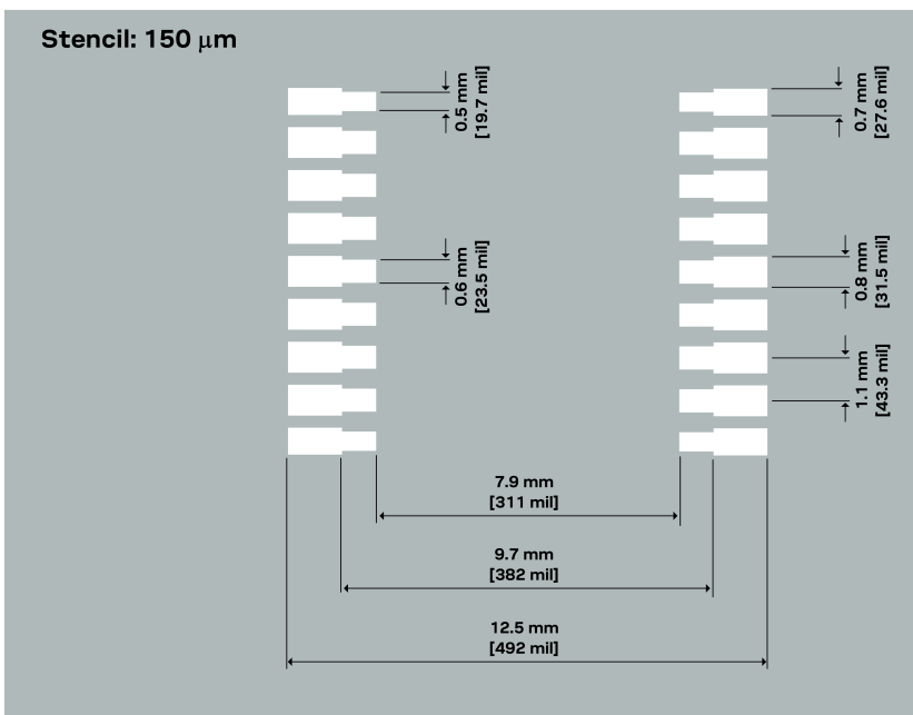
Figure 31: Recommended paste mask pattern for MAX-M10S
