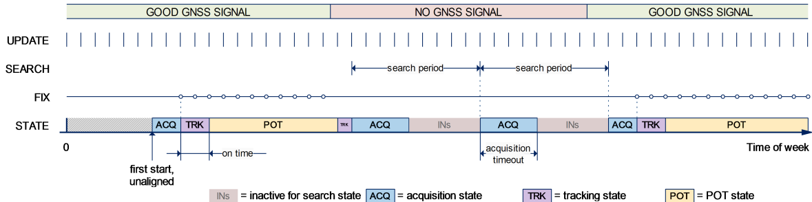
Figure 13: Cyclic tracking operation
