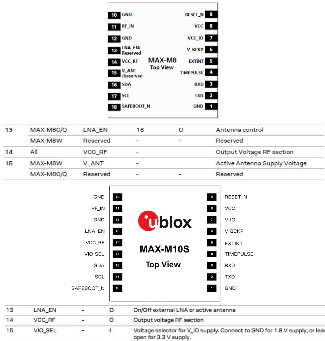
Figure 35: MAX-M8 vs. MAX-M10S comparison (pin 13 - 15)
