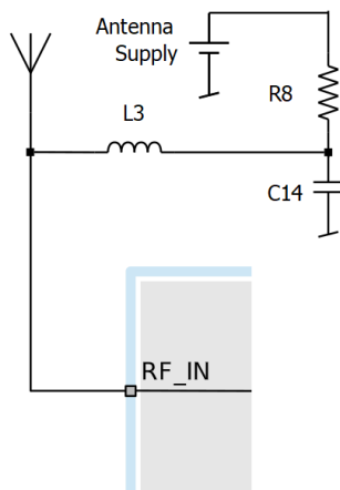
Figure 27: Antenna supply network
