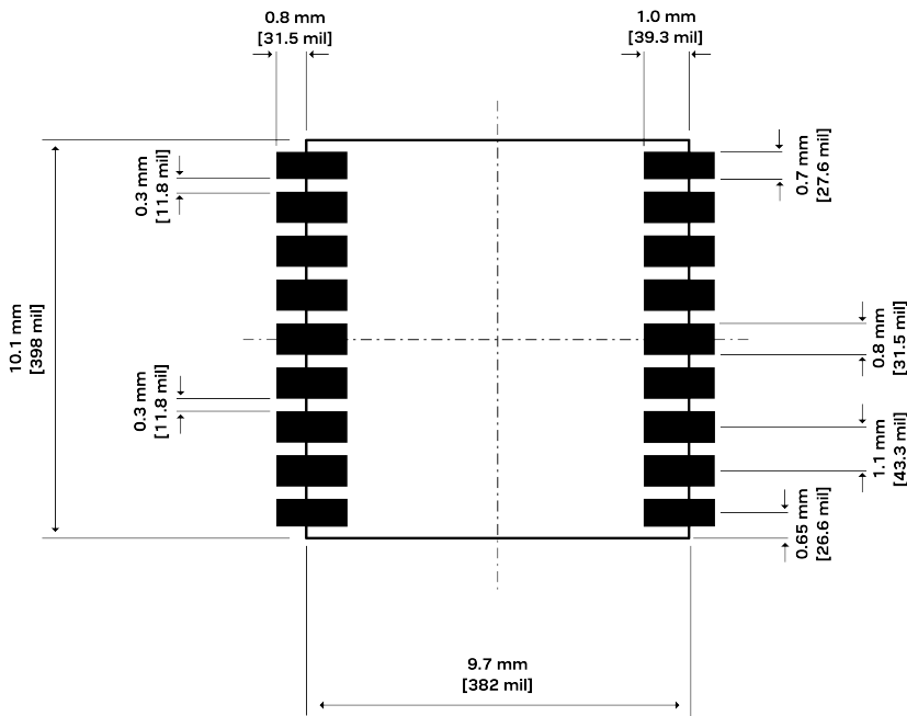
Figure 30: Recommended copper land and solder mask opening for MAX-M10S
