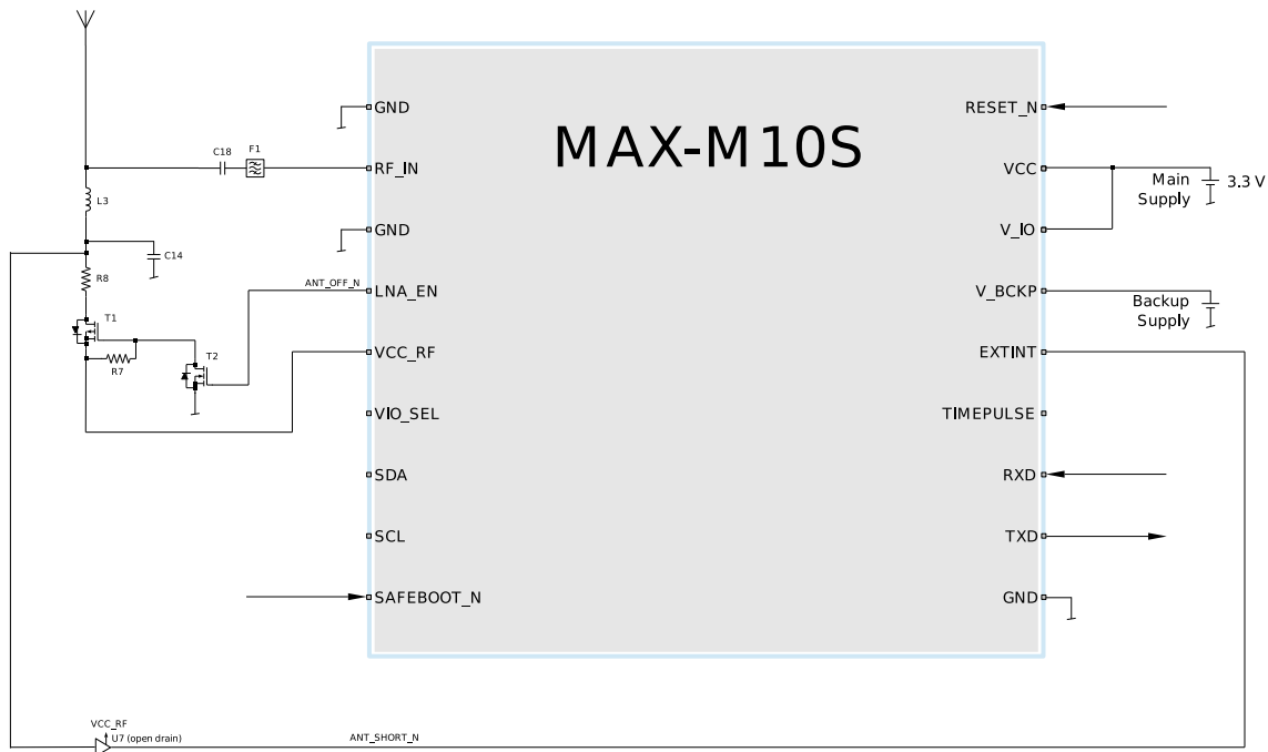
Figure 38: 2-pin antenna supervisor design
