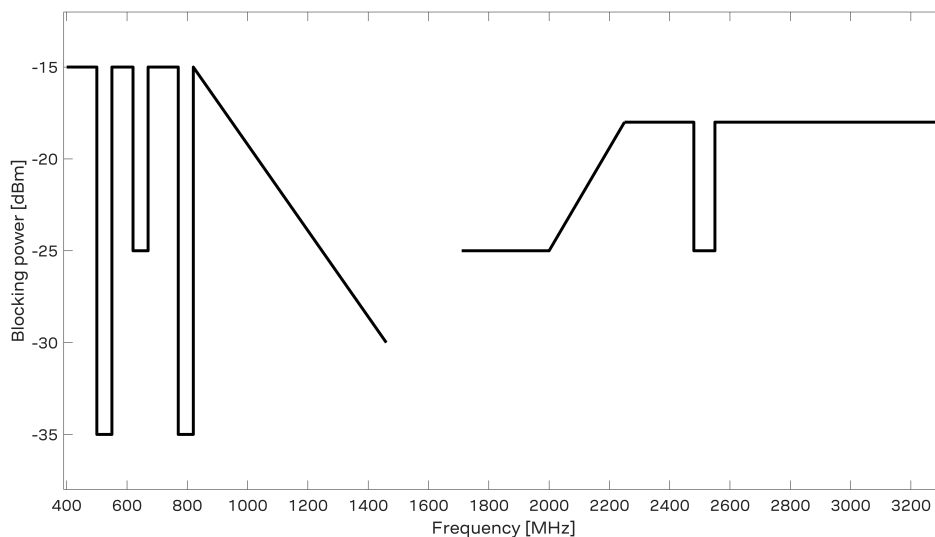
Figure 26: MAX-M10S out-of-band immunity level at 400 - 1460 MHz and 1710 - 3300 MHz for the low-gain mode (default).
