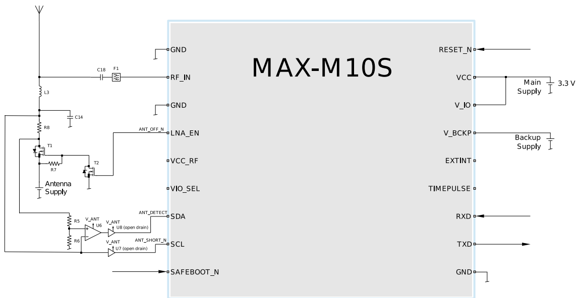
Figure 39: 3-pin antenna supervisor design
