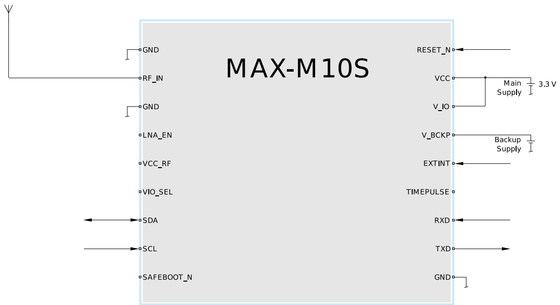
Figure 36: Typical 3.3 V design
