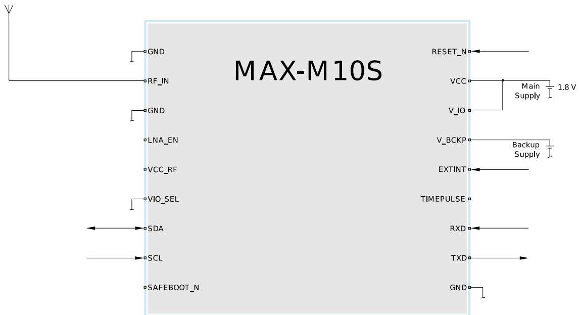
Figure 37: Typical 1.8 V design
