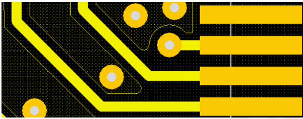
Figure 28: GND stub ended with a via
