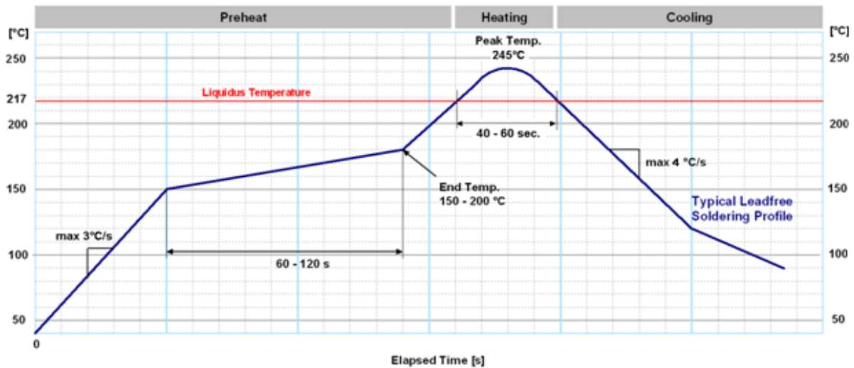
Figure 34: Soldering profile
